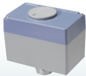
SQS65.5U 24 Vac Modulating, Spring Return Electronic MT Series Valve Actuator
